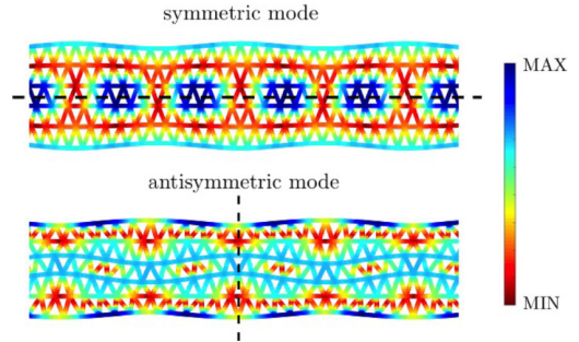
Figure: Lamb wave modes intensity, taken from cartaLambWavesDiscrete2023
