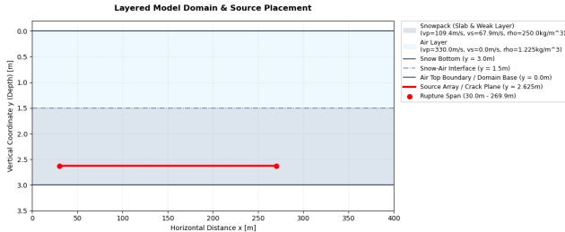
Figure: Two-layer model setup in SALVUS. Colors show materials, material types and properties in legend. Moving source line extent in red. Propagation speeds according to trottetTransitionSubRayleighAnticrack2022 .
